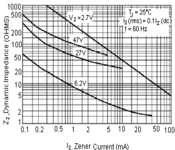
Effect of Zener Current on Zener Impedance
