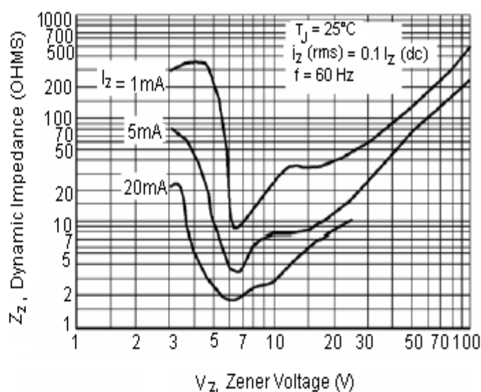
Effect of Zener Voltage on Zener Impedance
