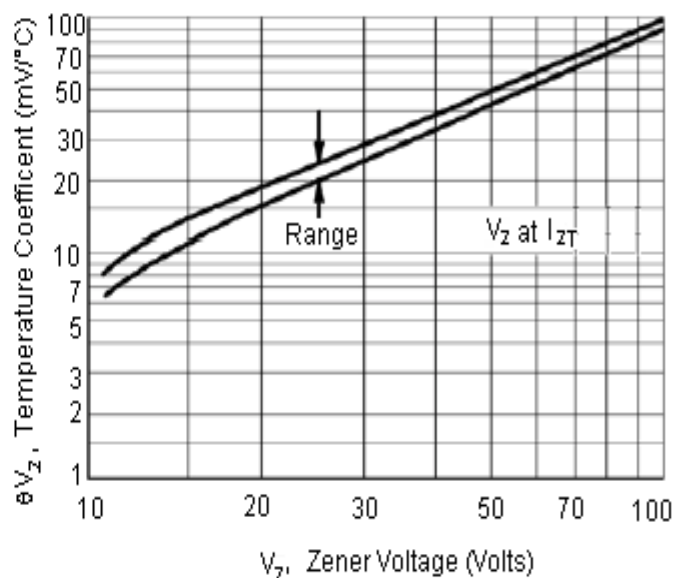
Temperature Coefficients
