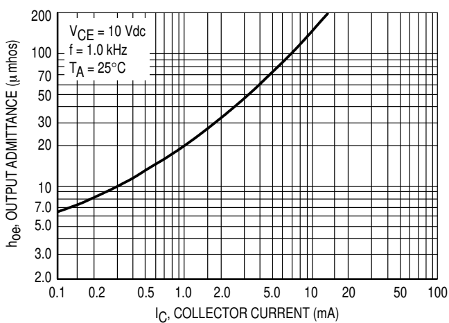
Figure 16. Output Admittance
