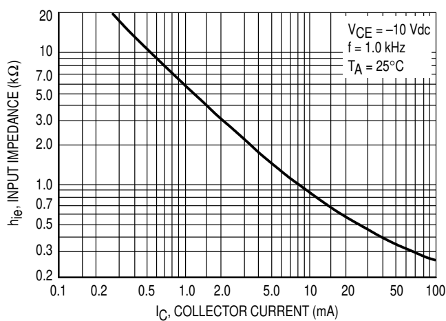
Figure 15. Input Impedance
