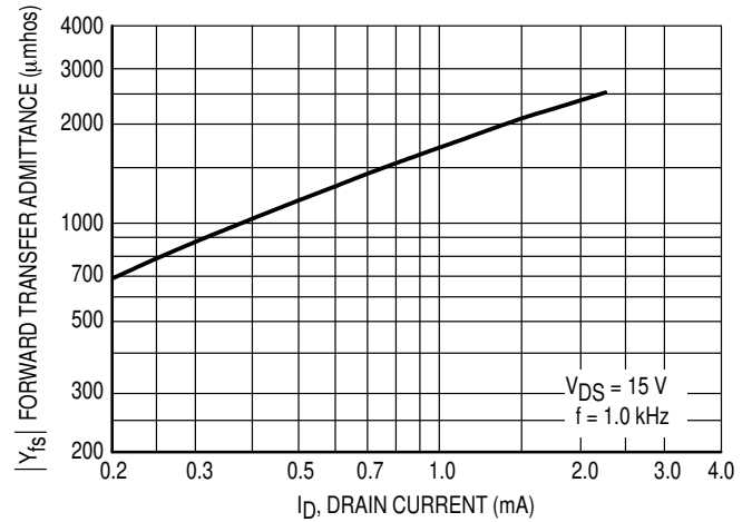
Figure 4. V_{GS(off)} = 2.0 Volts
