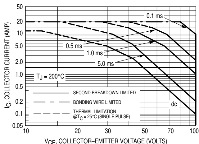
Figure 6. 2N6052, 2N6059
