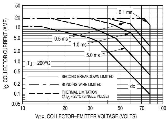
Figure 5. 2N6058
