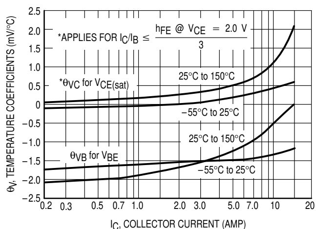
Figure 4. Temperature Coefficients
