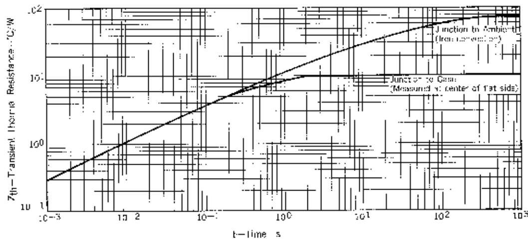
Fig. 11 Z_{th} CHARACTERISTICS
