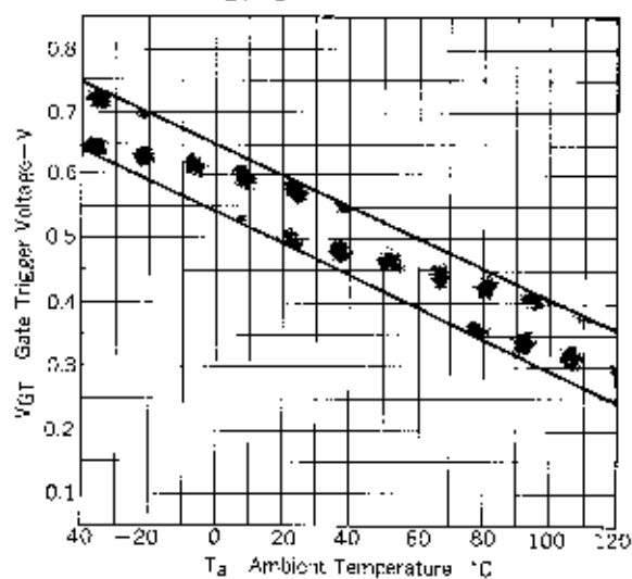
Fig. 6 V_{GT} - T_a TYPICAL DISTRIBUTION
