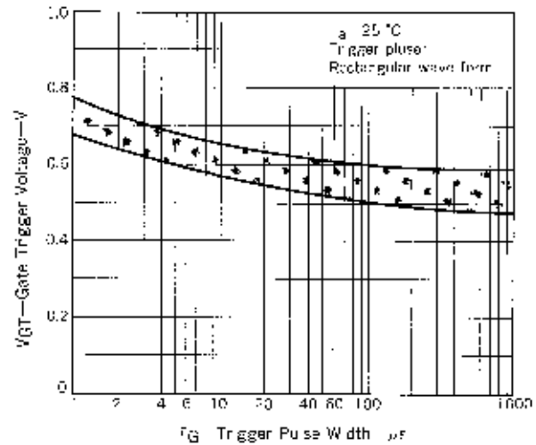
Fig. 8 V_{GT} t_G TYPICAL DISTRIBUTION
