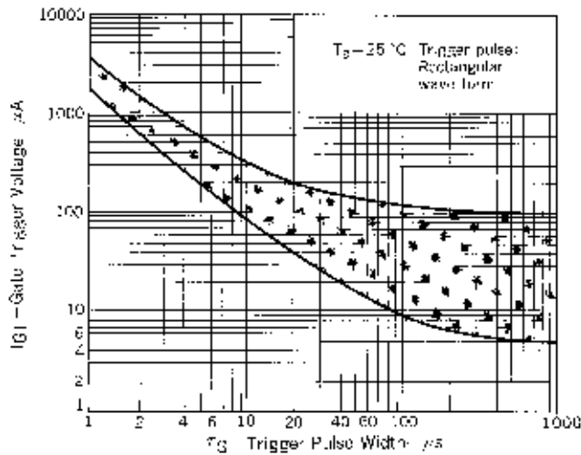
Fig. 7 I_{GT} t_G TYPICAL DISTRIBUTION
