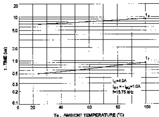
SWITCHING TIME- AMBIENT TEMPERATURE
