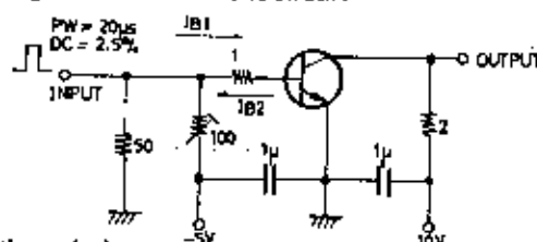
Switching time measurement circuit
