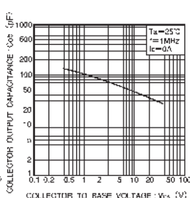
Fig.9 Collector output capacitance vs. collector-base voltage
