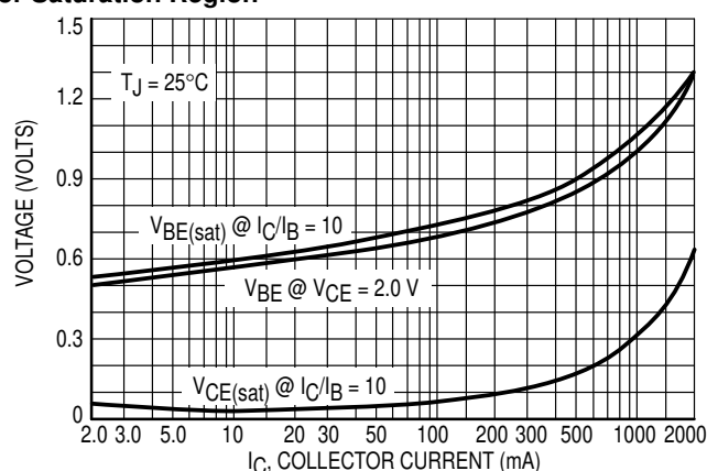
Figure 4. "On" Voltages
