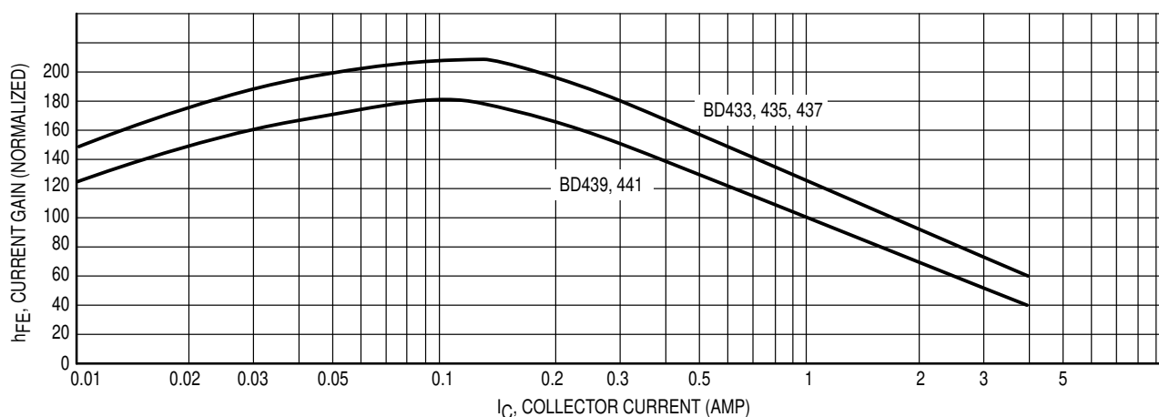
Figure 2. Current Gain
