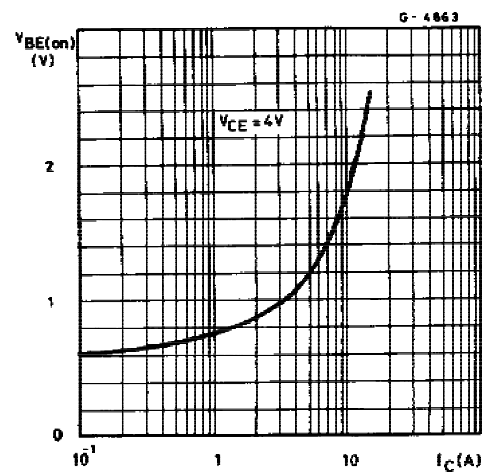
DC Transconductance(NPN type)
