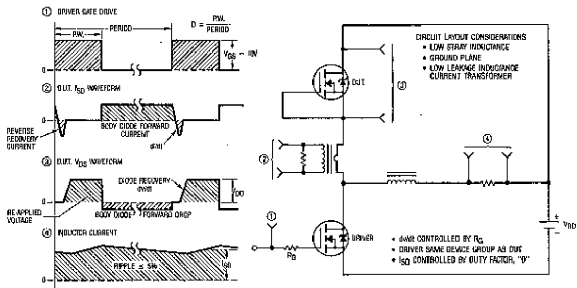
Fig. 17 — Peak Diode Recovery \frac{dv}{dt} Test Circuit
