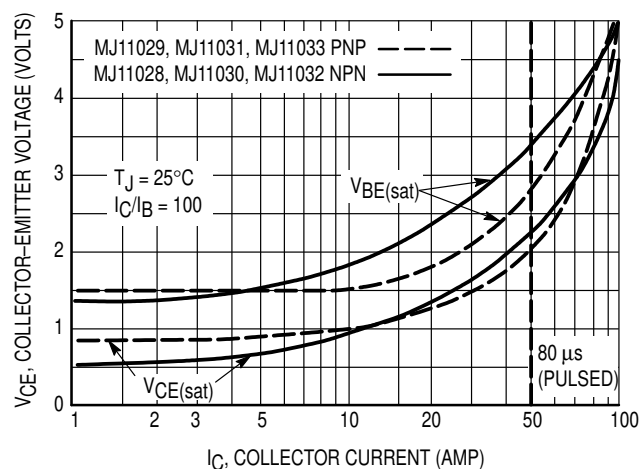
Figure 4. "On" Voltage
