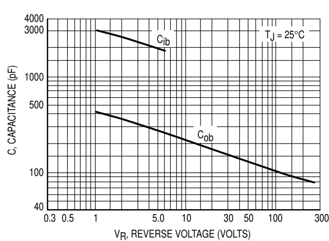
Figure 2. Capacitances
