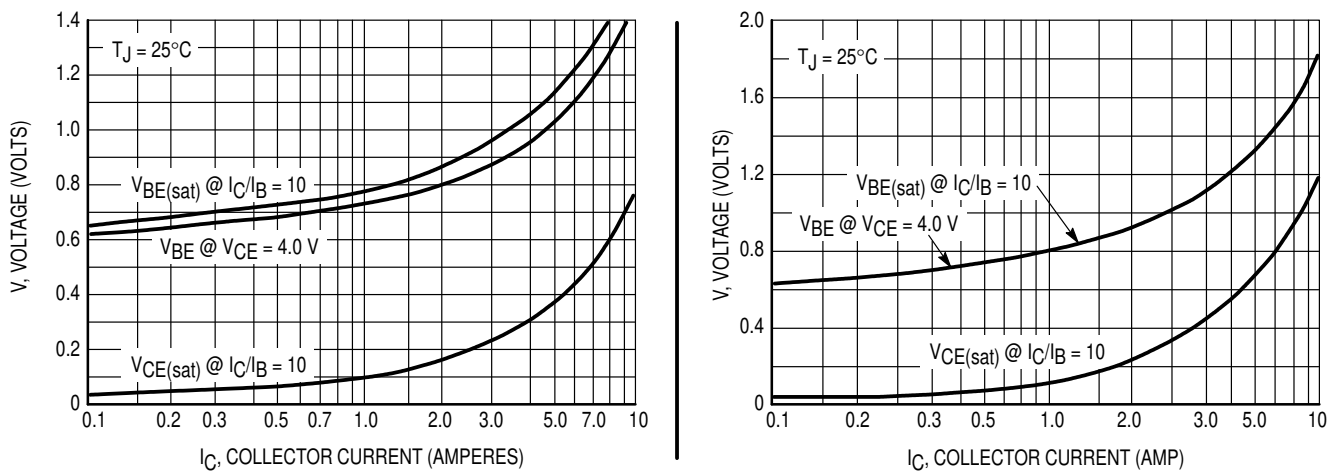
Figure 5. "On" Voltages
