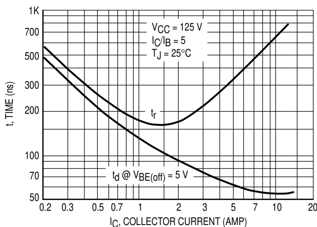
Figure 11. Turn-On Time
