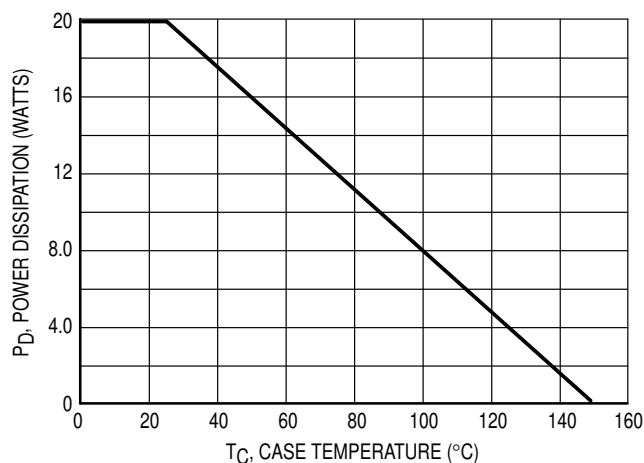
Figure 5. Power Derating
