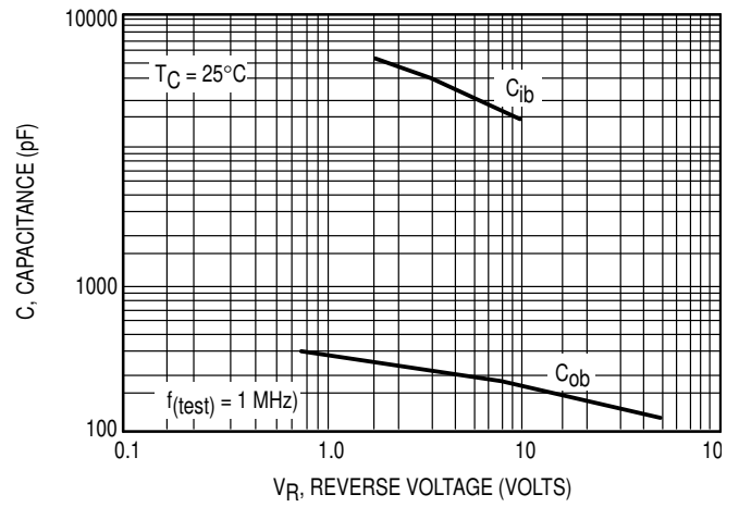
Figure 15. MJL21194 Typical Capacitance
