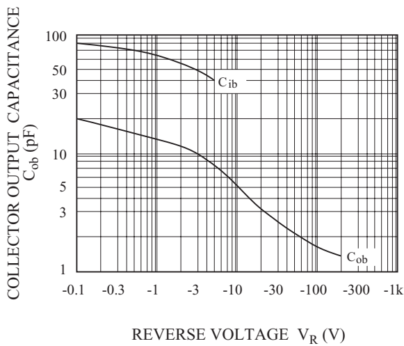
C_{ob} - V_R
