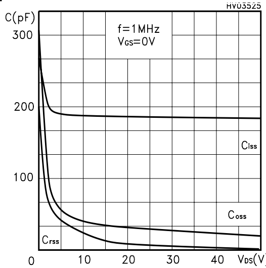
Capacitance Variations
