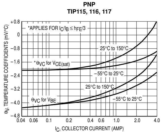
Figure 11. Temperature Coefficients
