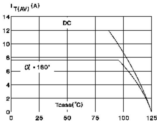
Fig.6 : Average on-state current versus case temperature (TYN).
