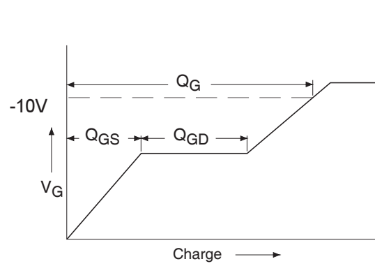
Fig 12a. Basic Gate Charge Waveform
