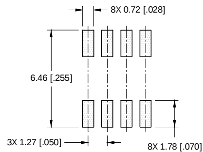
FOOTPRINT
