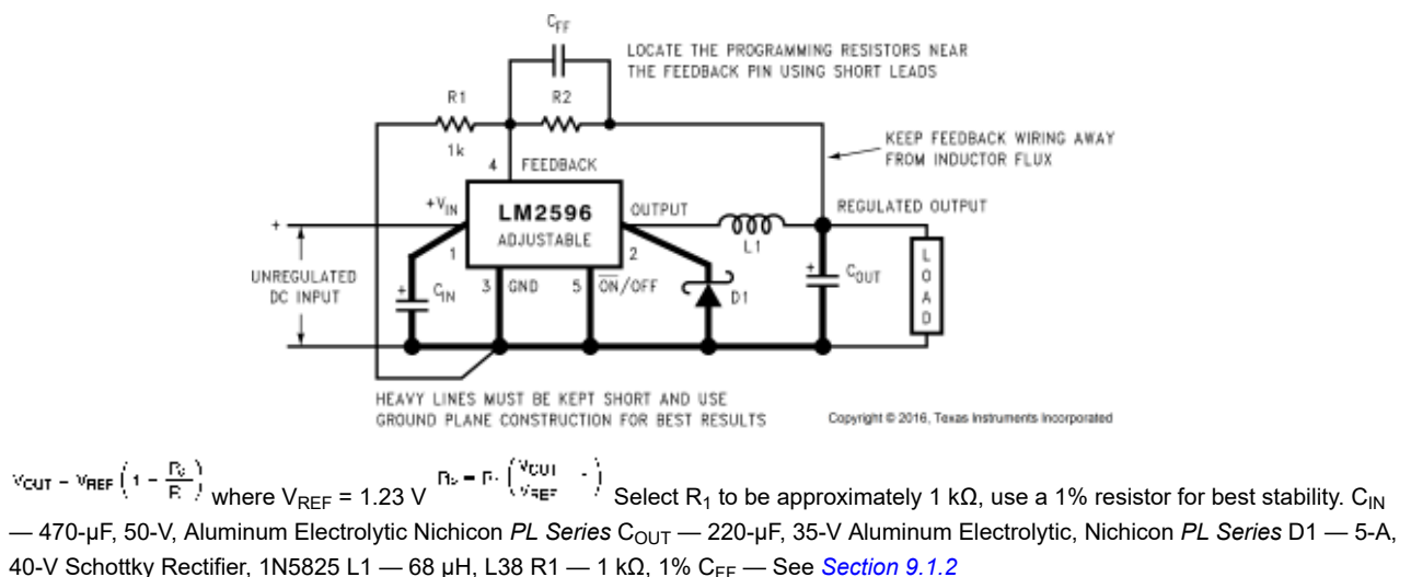
Figure 9-13. Adjustable Output Voltage Version
