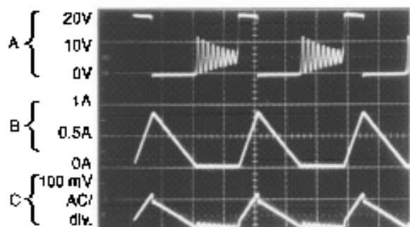
Discontinuous Mode Switching Waveforms V_{\text{IN}} = 20\text{ V} , V_{\text{OUT}} = 5\text{ V} , I_{\text{LOAD}} = 500\text{ mA} , L = 10\text{ }\mu\text{H} , C_{\text{OUT}} = 330\text{ }\mu\text{F} , C_{\text{OUT}} \text{ ESR} = 45\text{ m}\Omega
