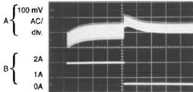
Load Transient Response for Discontinuous Mode V_{\text{IN}} = 20\text{ V} , V_{\text{OUT}} = 5\text{ V} , I_{\text{LOAD}} = 500\text{ mA} to 2 A, L = 10\text{ }\mu\text{H} , C_{\text{OUT}} = 330\text{ }\mu\text{F} , C_{\text{OUT}} \text{ ESR} = 45\text{ m}\Omega
