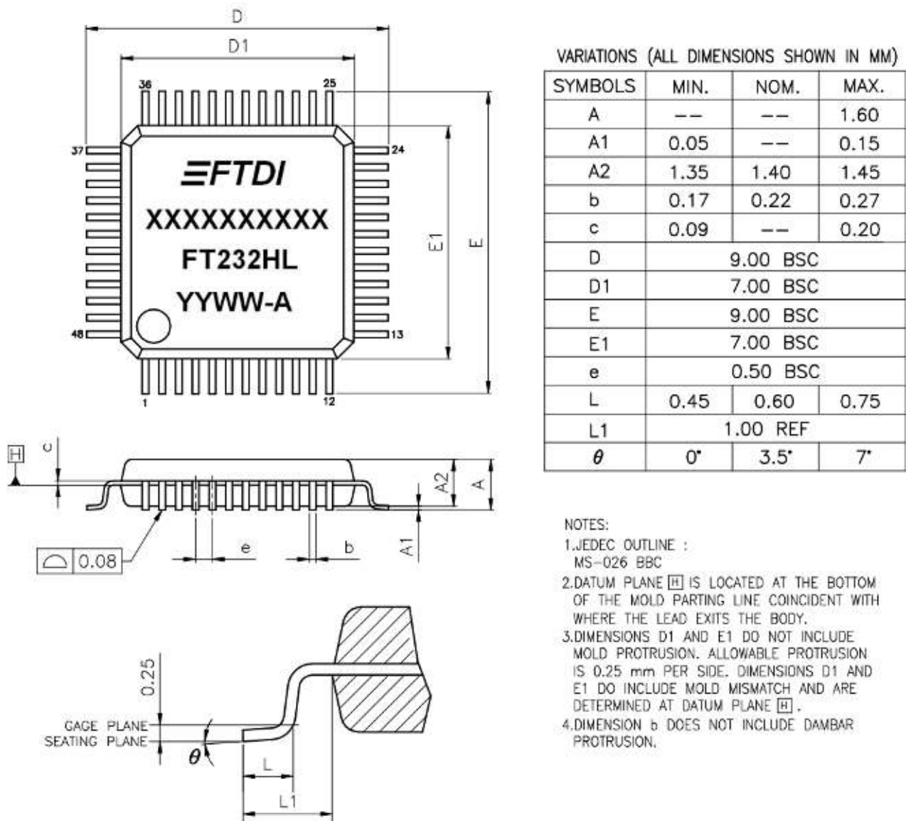
Figure 8.2 48 pin LQFP Package Details
