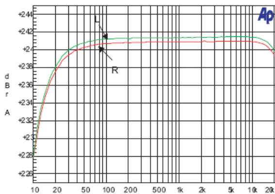
5. Frequency response
