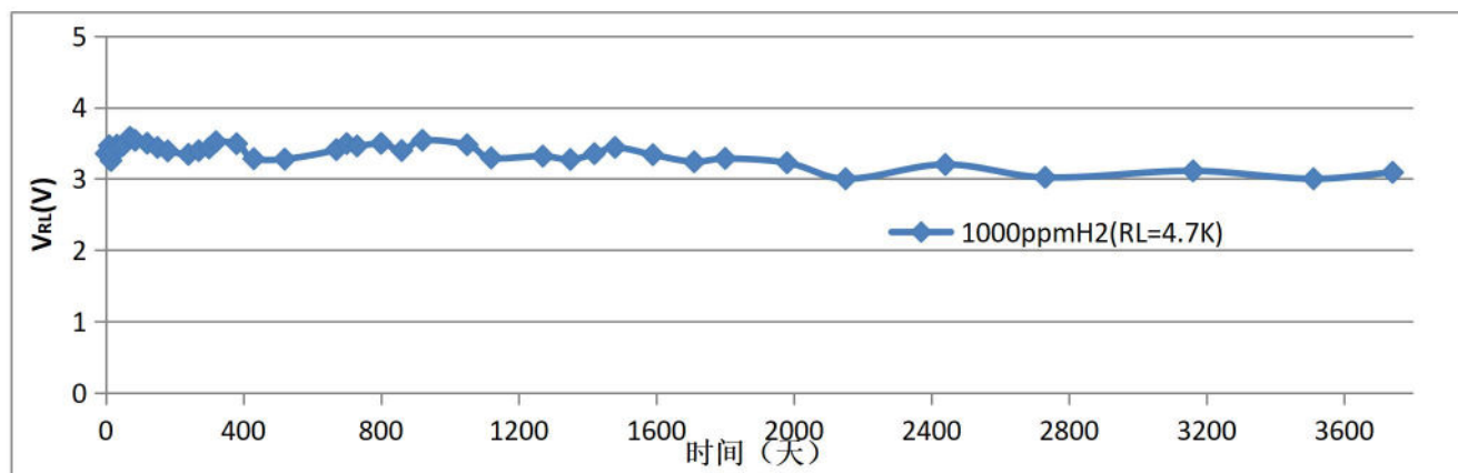
Fig7. long-term Stability
