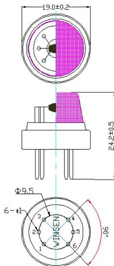
Fig1.Sensor Structure
