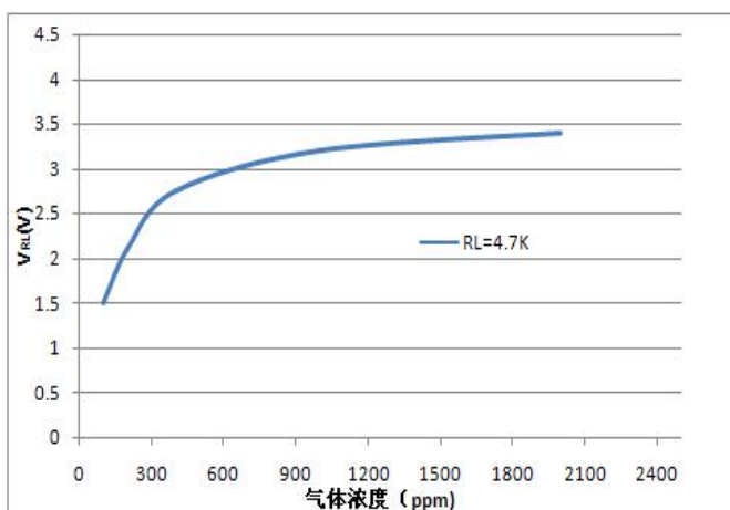
Fig5. Sensitivity Curve
