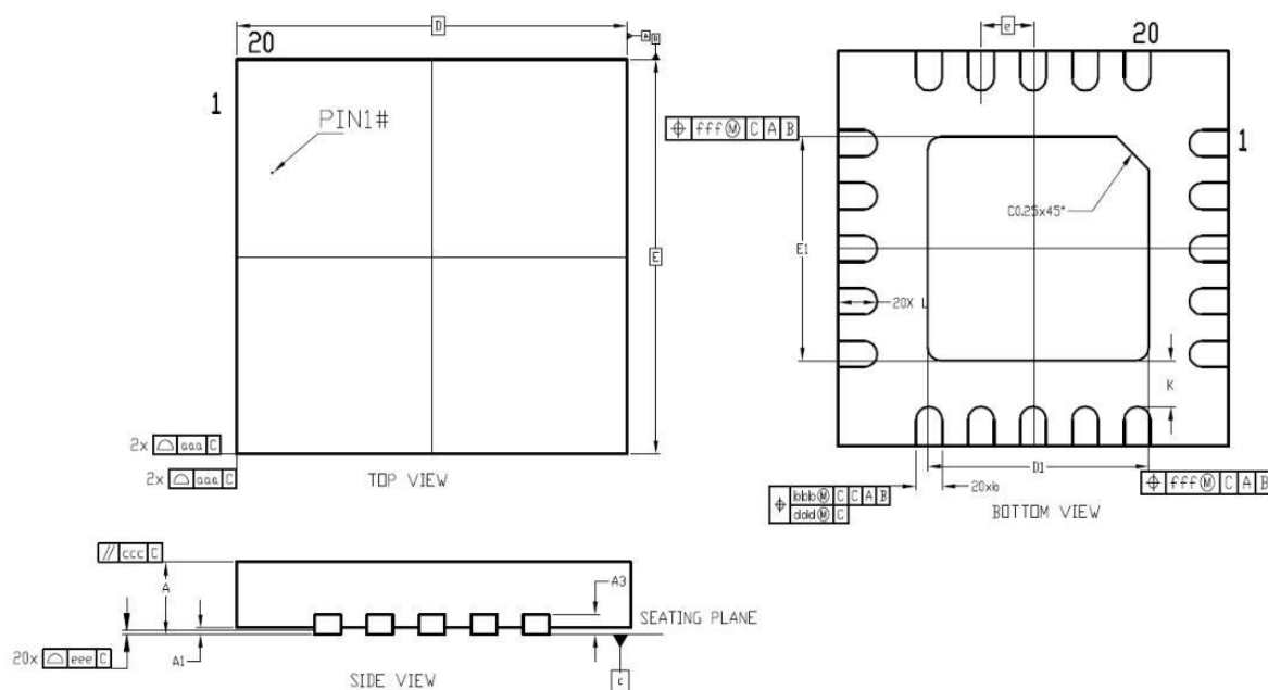
Figure 10 QFN20 Outline Drawing
