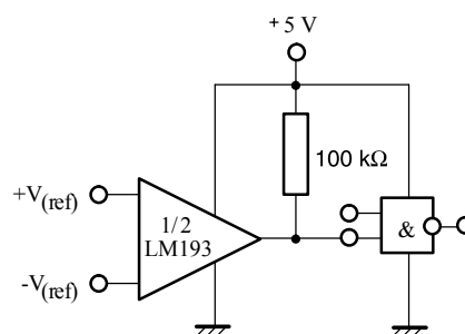
Figure 12. Driving CMOS
