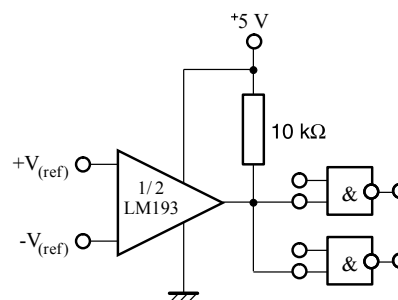
Figure 10. Driving TTL
