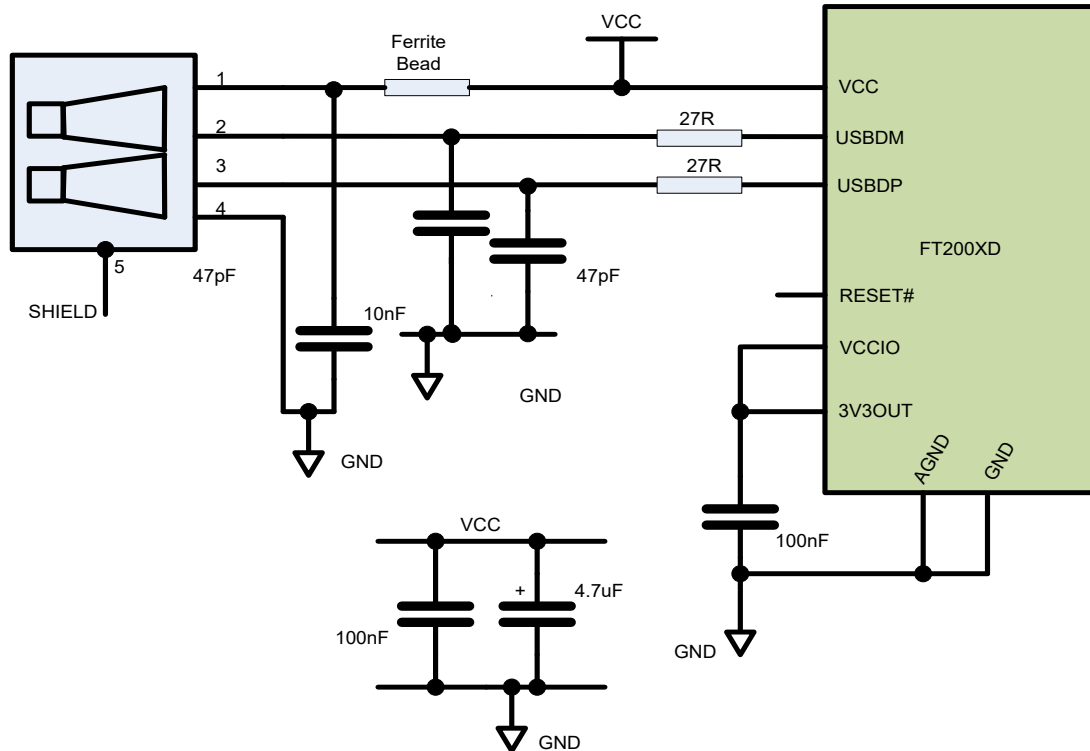
Figure 7.1 Bus Powered Configuration
