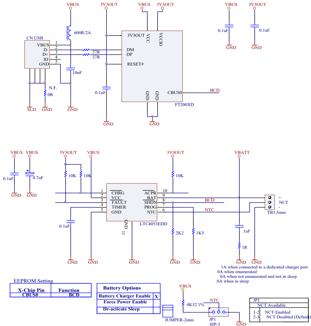
Figure 8.2 USB Battery Charging Detection
